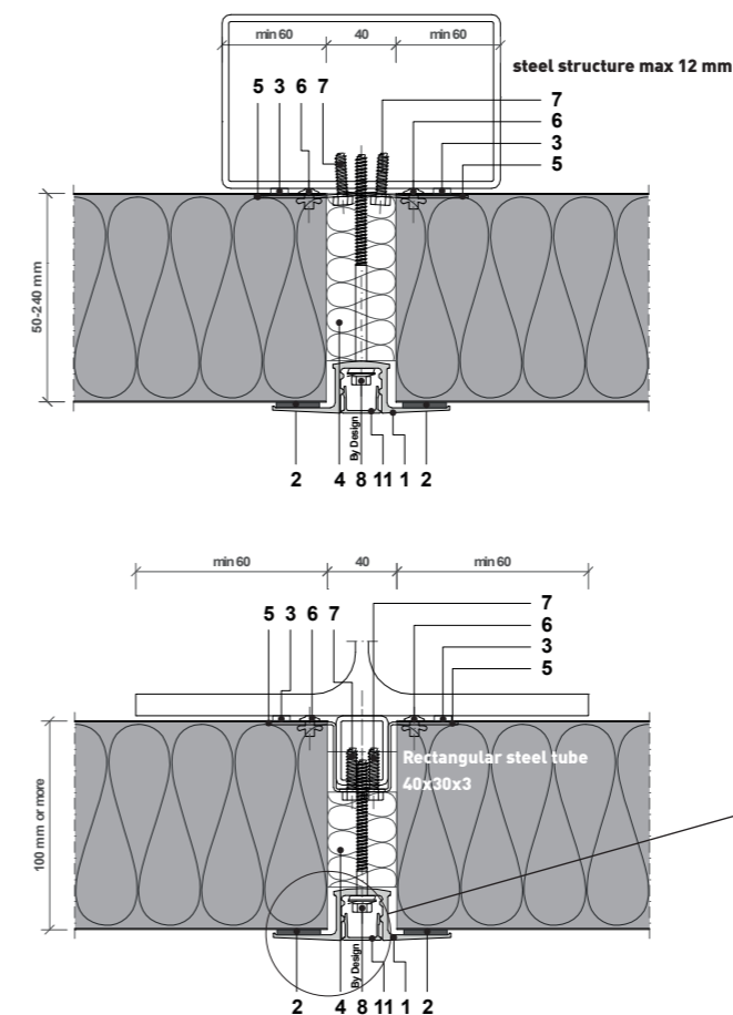
Fig. 11: Fixing of a horizontal façade to a steel structure, depends on the thickness of substructure
