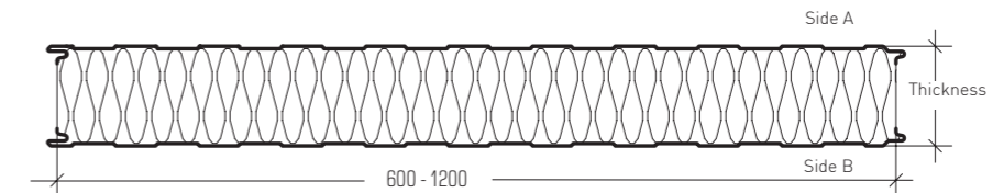
Fig. 1: Trimoterm FTV façade panels
