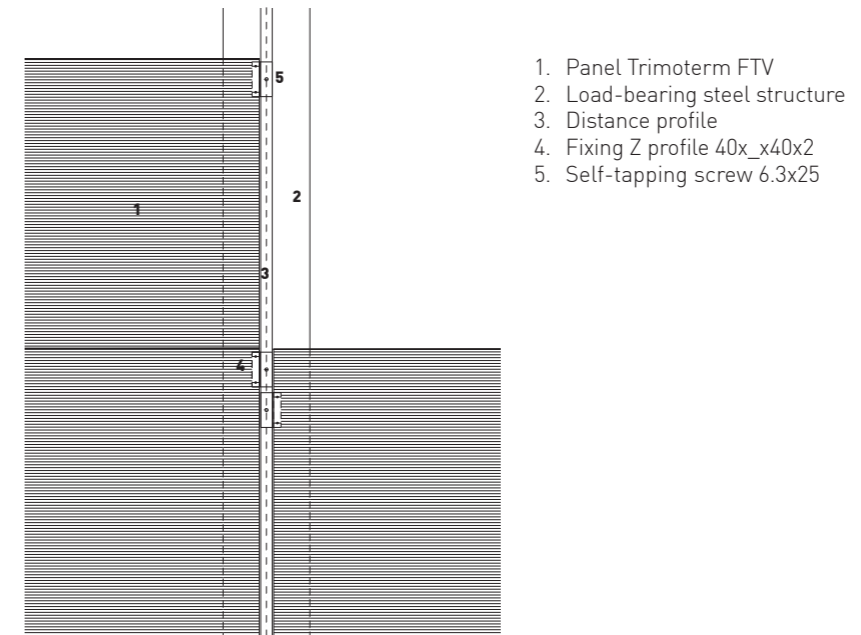
Fig. 17: Temporary mounting (1 piece / panel)
