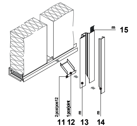
Trimoterm FTV base detail 3D view
