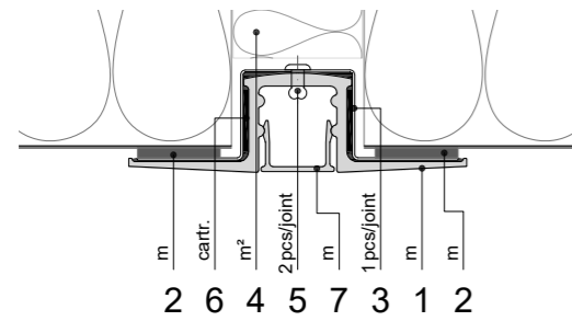
Fig. 18: Position of sealing tape on the HF102 aluminium profile
