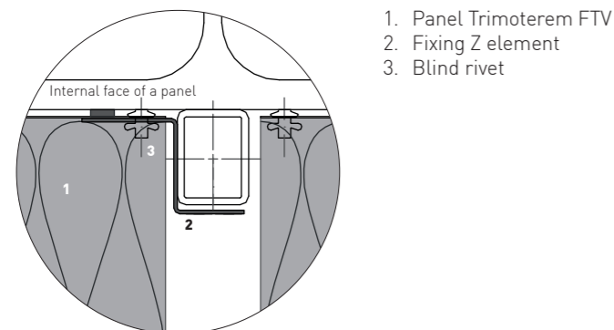
Fig. 13: Temporary mounting
