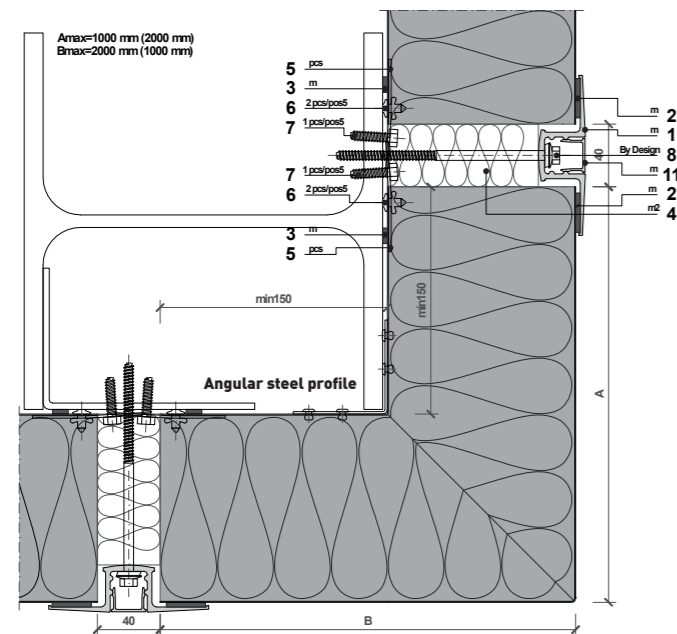
Fig. 9: Preformed sharp-edged corner
