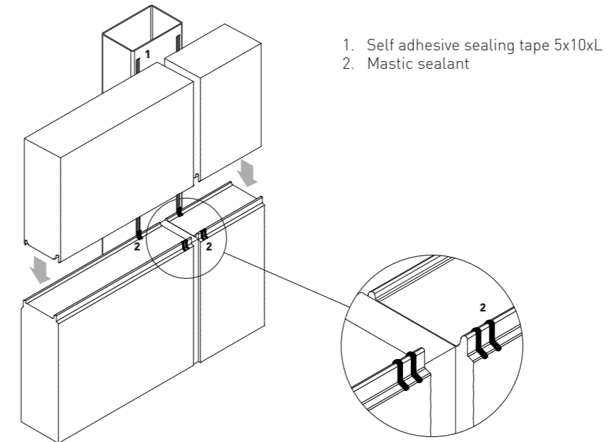
Fig. 2a: Position of sealing components
